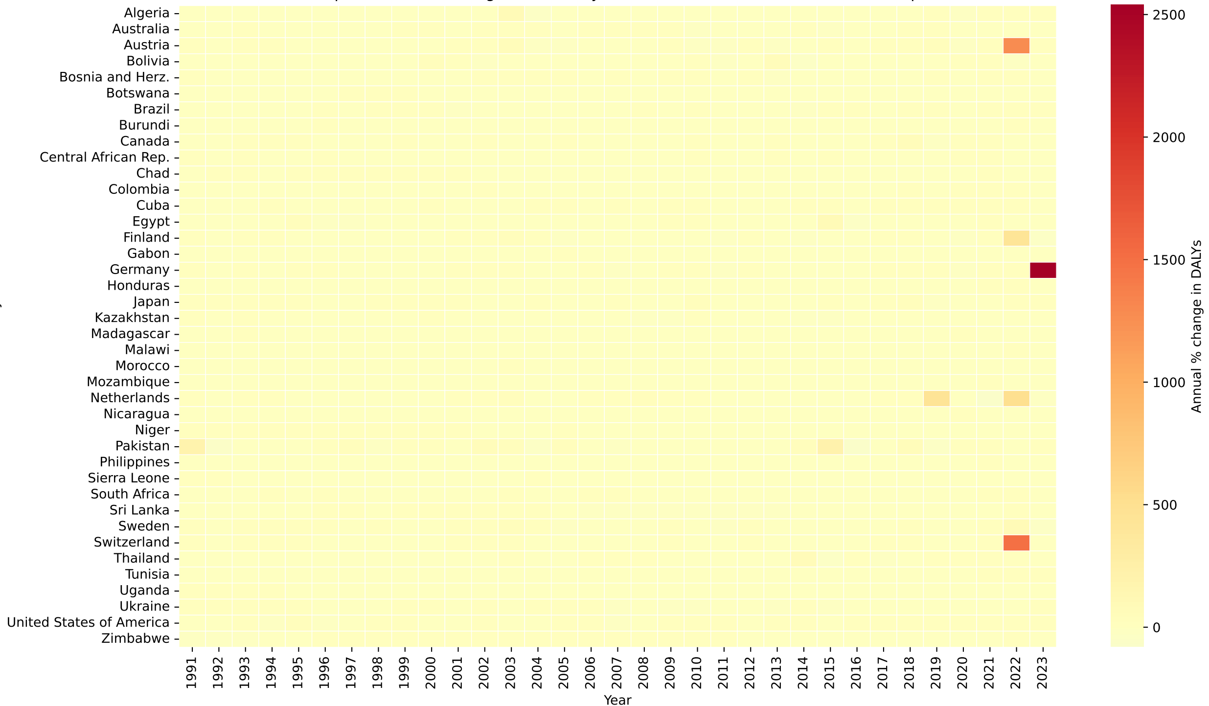
Heat map of annual % change in DALYs by cause 'Environmental heat and cold exposure'
